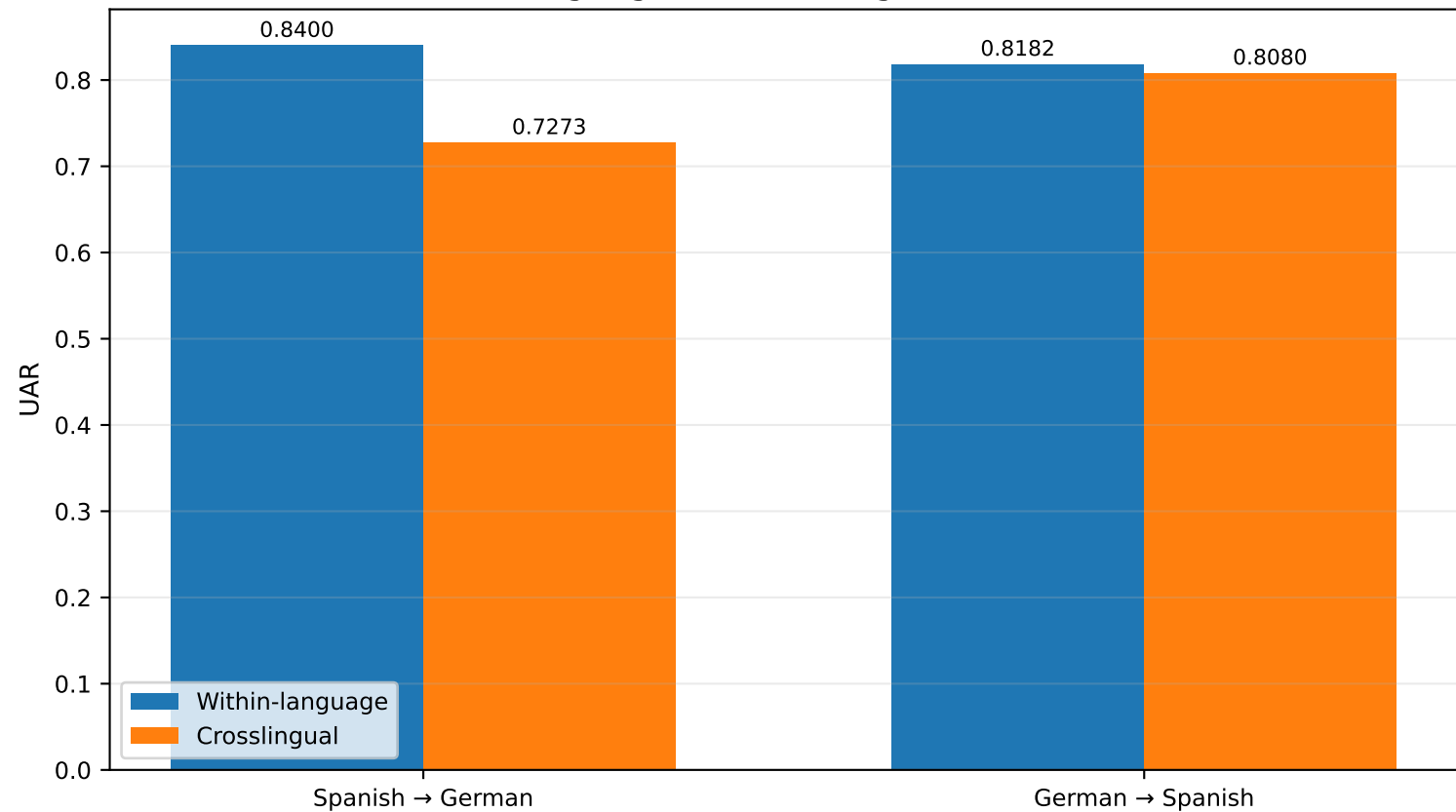
Within-Language vs. Crosslingual Baseline UAR
