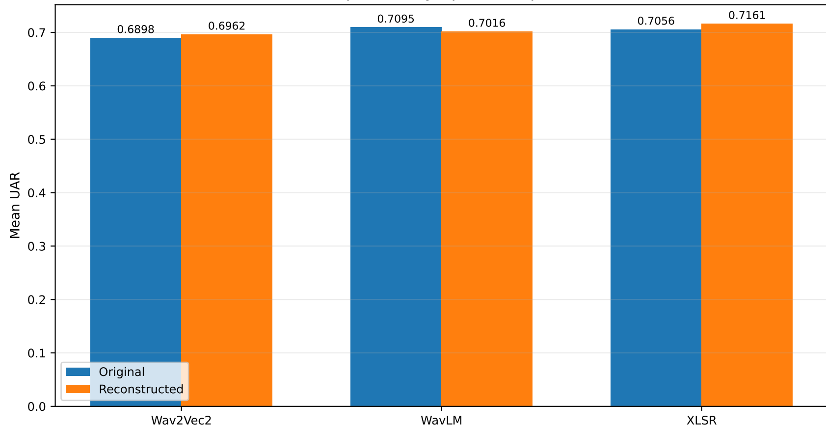
Classification Comparison by Speech Representation Model
