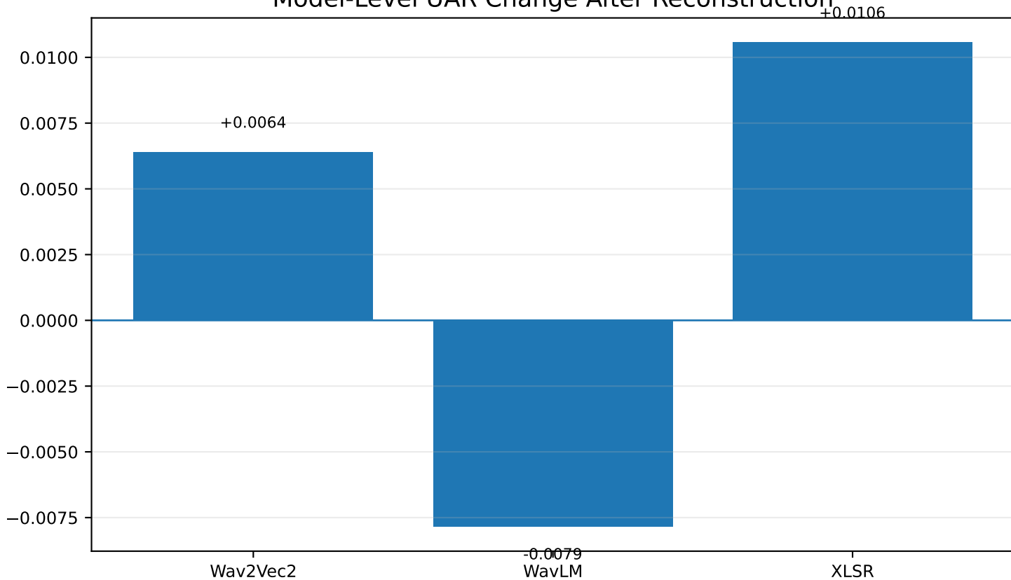
Model-Level UAR Change After Reconstruction
