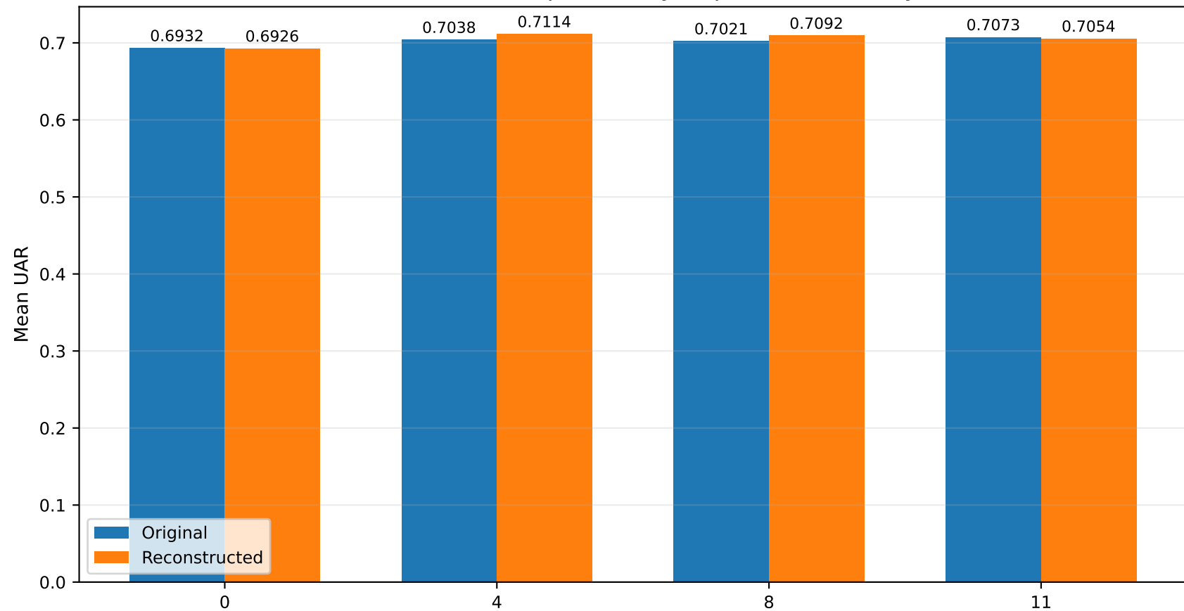
Classification Comparison by Representation Layer
