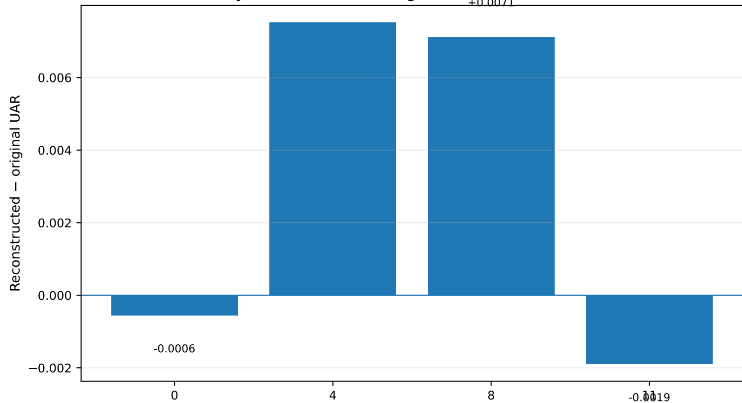
Layer-Level UAR Change After Reconstruction
