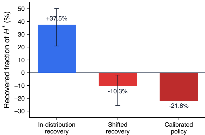
B. Recoverable headroom under shift (shift AUC = 0.957)
