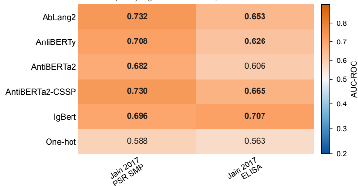
a Jain 2017 clinical panel - AUC-ROC Jain developability flags: PSR SMP < 0.27; ELISA < 1.9
