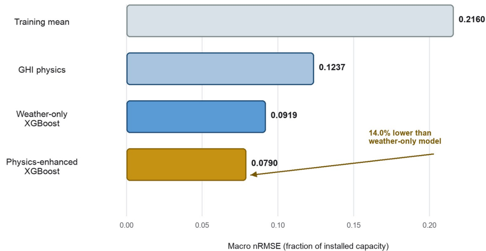
Figure 2. Macro nRMSE across four models. Errors are calculated on capacity-normalized power for each held-out system and then averaged equally across 37 systems. Lower values indicate better cross-system prediction. The hybrid value is 14.0% below the weather-only value. Source: Project Phase 3 results and executed Phase 4 notebook output.
