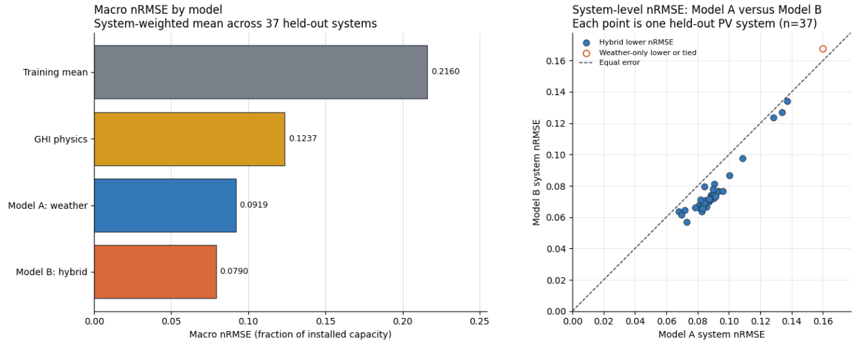
Figure 2. Same-period model comparison. The left panel shows macro nRMSE across the four models. The right panel compares weather-only Model A with physics-enhanced Model B for each held-out PV system; points below the identity line favor Model B. Model B has lower nRMSE on 36 of 37 systems. Source: Study analysis outputs.
