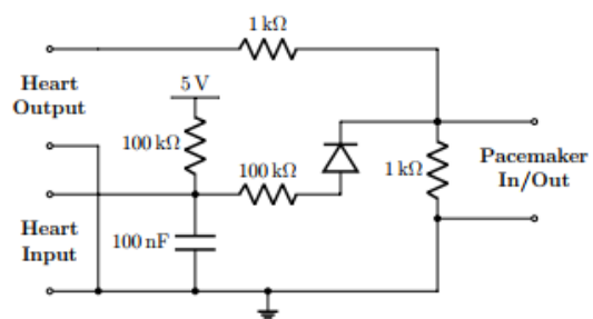
Figure 6.9: The interface that connects the pacemaker to the emulated heart
