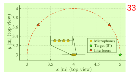
Fig. 1: Top view of the simulated acoustic scene. 34
