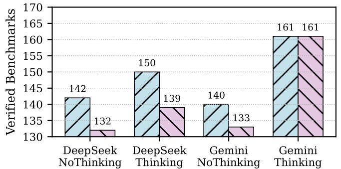
(a) Progressive vs Unified (Diagnostic Message)
