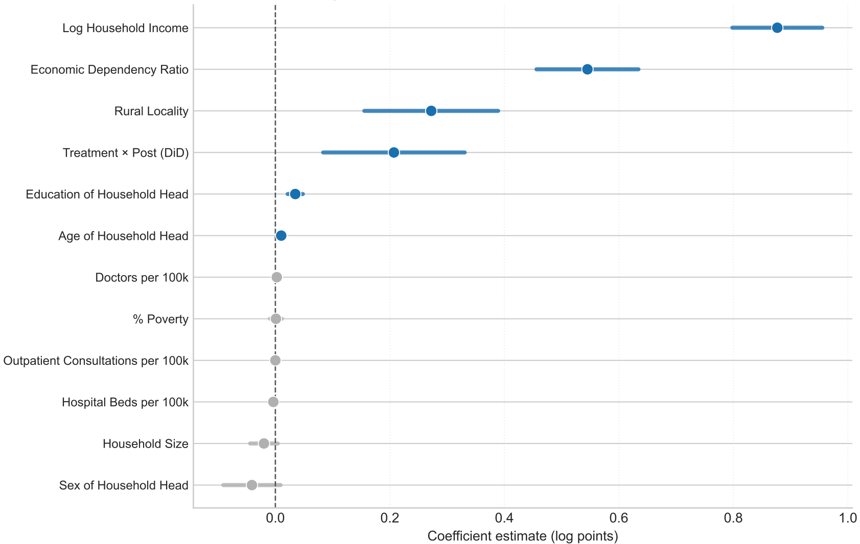
Figure A2. Full Covariate Effects — Main PPML Model
