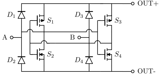
Figure 4.2: Negative voltage converter used for one of the three two-phase groups of pickup units, with phase terminals A , B .
