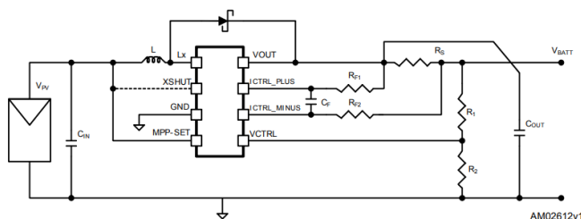
Figure 9.5: SPV1040 block diagram.
