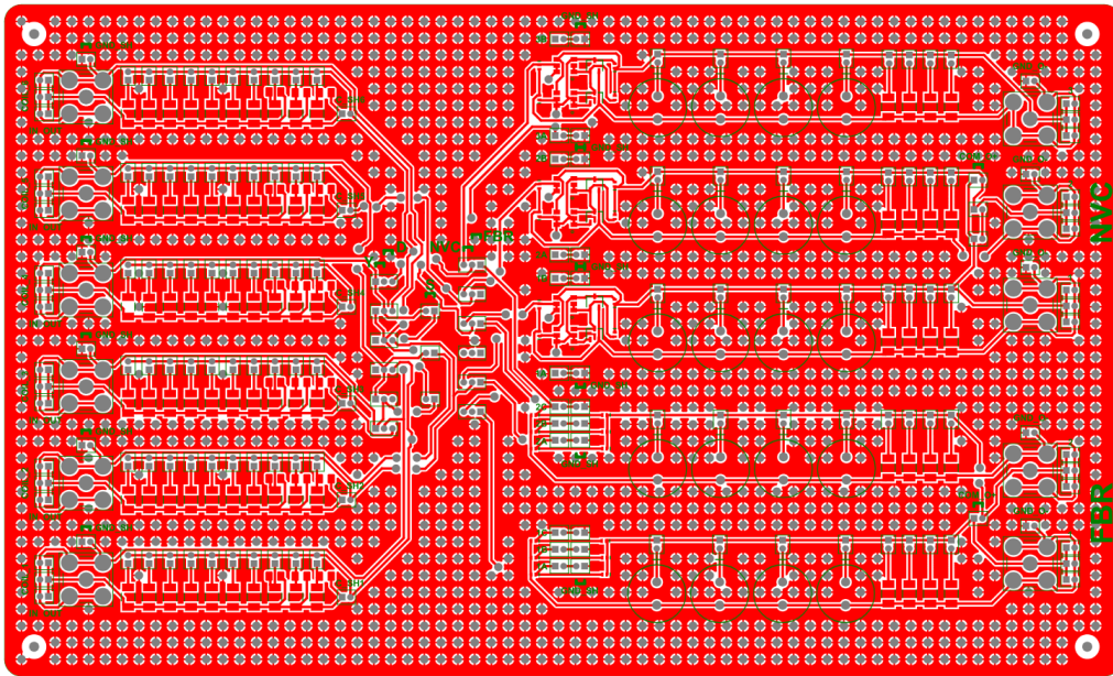
(a) Top copper layer.
