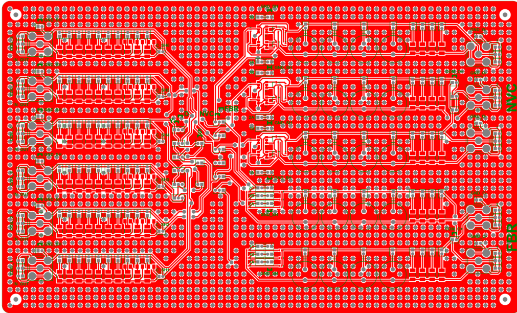
(a) Top copper layer.
