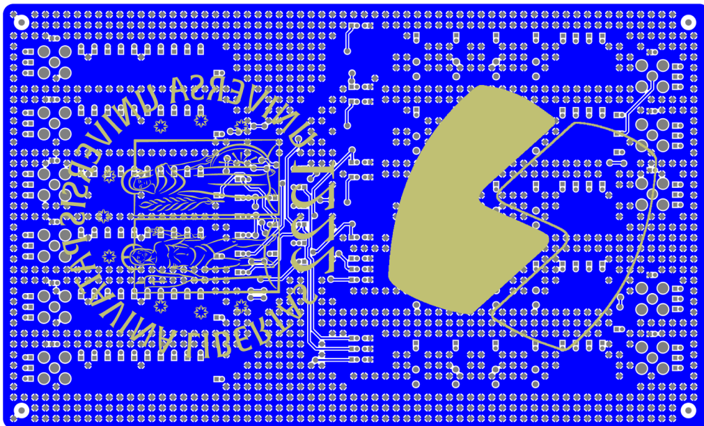
(b) Bottom copper layer.
