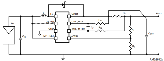
Figure 9.5: SPV1040 block diagram.
