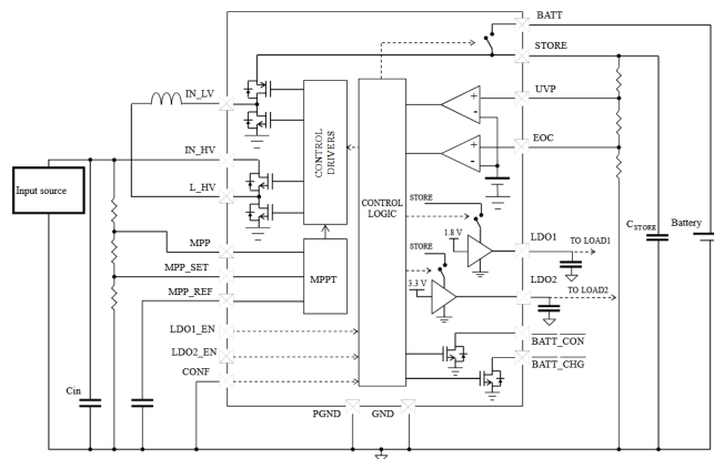
Figure 9.4: SPV1050 block diagram.
