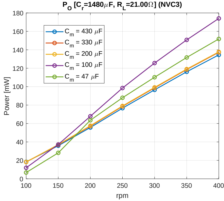
Figure 7.22: Output power of NVC3 across the target speed range, for five fixed values of the compensation capacitor C_m ( C_r = 1480 \mu\text{F} , R_L = 21 \Omega ).
