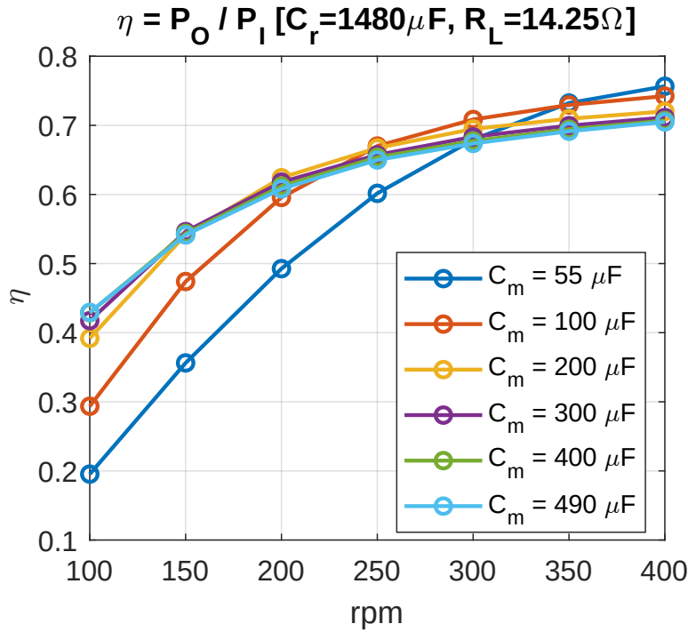
Figure 4.9: Power conversion efficiency (PCE) of the first and second bridges combined, across the target speed range, for six fixed values of the compensation capacitor C_m ( C_r = 1480 \mu F , R_L = 14.25 \Omega ).
