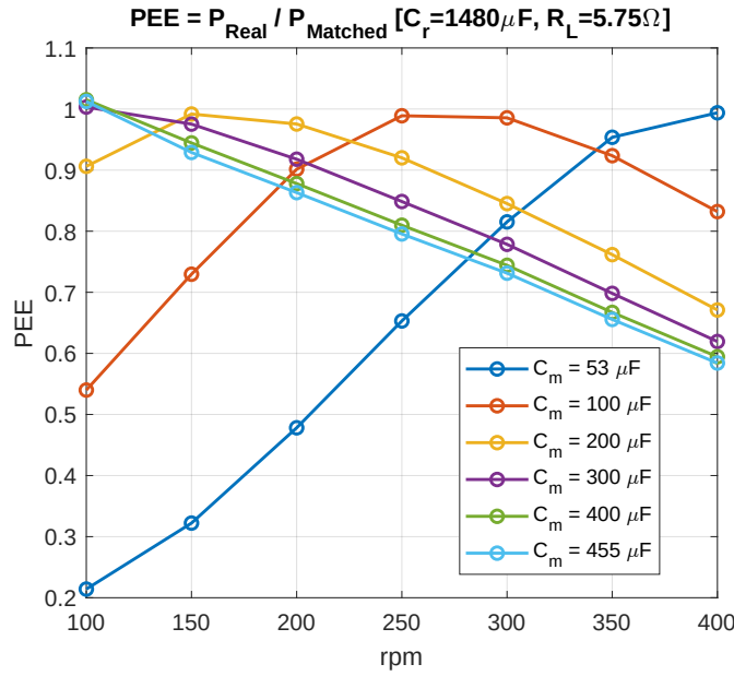
Figure 4.17: Power extraction efficiency (PEE) of the first and second bridges combined, across the target speed range, for six fixed values of the compensation capacitor C_m ( C_r = 1480 \mu F , R_L = 5.75 \Omega ).
