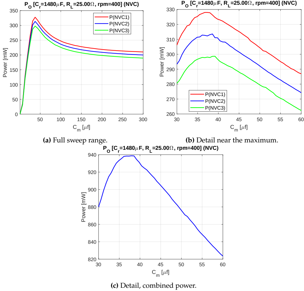
Figure 4.19: Output power of the three NVC bridges as a function of the compensation capacitor C_m at 400 rpm ( C_r = 1480 \mu\text{F} , R_L = 25.00 \Omega ), shown individually (a, b) and combined (c).
