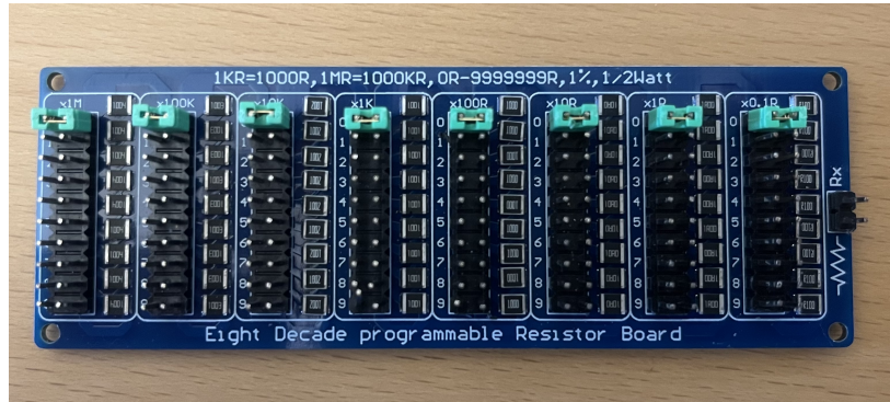
Figure 6.6: The eight-decade programmable resistor board used to set the load resistance R_L .
