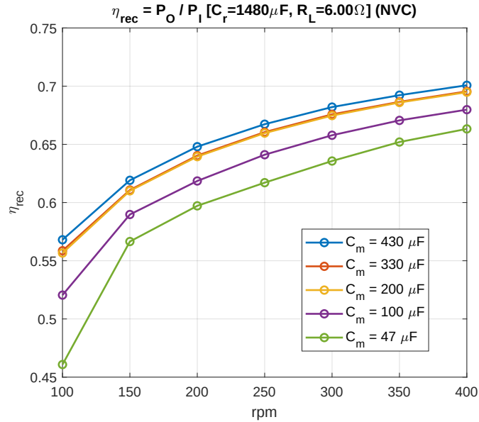
Figure 7.24: Rectifier efficiency \eta_{rec} of the three NVC bridges combined, already connected in parallel, across the target speed range, for five fixed values of the compensation capacitor C_m ( C_r = 1480 \mu F , R_L = 6 \Omega ).
