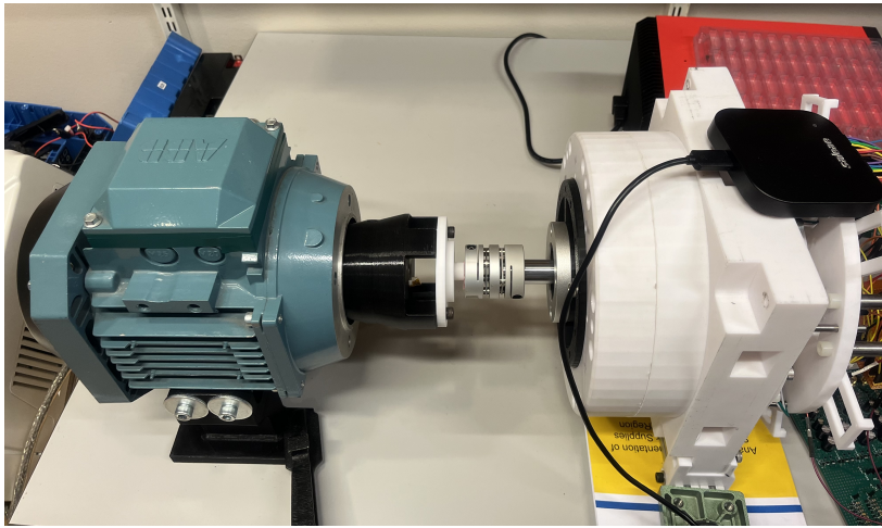
Figure 6.1: Test bench used for all measurements: the induction motor (left) coupled through a shaft coupling to the MP-VREH harvester (right, white housing).
