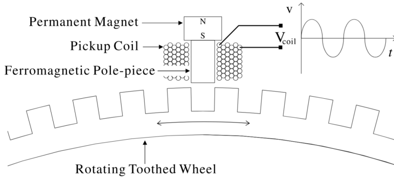
Figure 2.1: Structure of a variable-reluctance sensor
