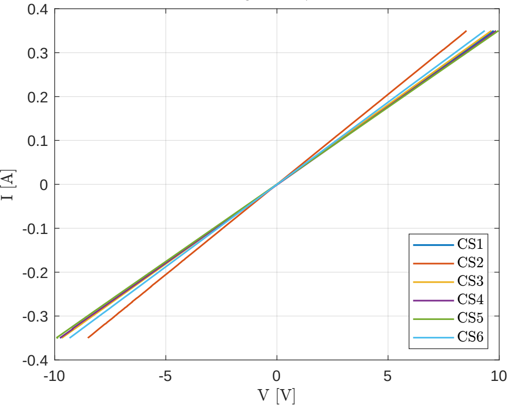
Curve I-V
