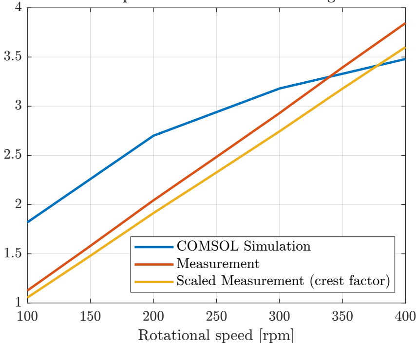
Comparison of Peak-to-Peak Voltage
