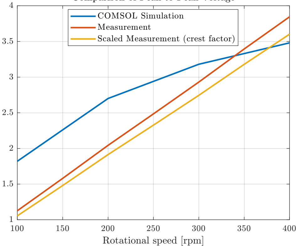
Comparison of Peak-to-Peak Voltage
