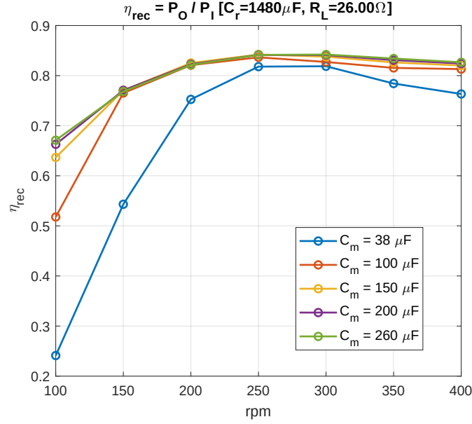
Figure 4.22: Rectifier efficiency \eta_{Rec} of the three NVC bridges combined, across the target speed range, for five fixed values of the compensation capacitor C_m ( C_r = 1480 \mu F , R_L = 26.00 \Omega ).
