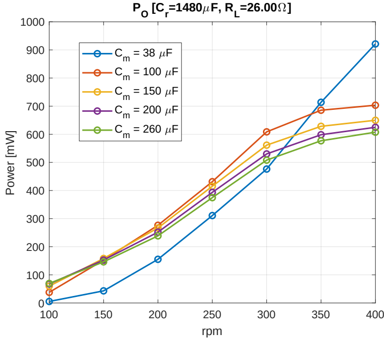
Figure 4.21: Combined output power of the three NVC bridges across the target speed range, for five fixed values of the compensation capacitor C_m ( C_r = 1480 \mu\text{F} , R_L = 26.00 \Omega ).
