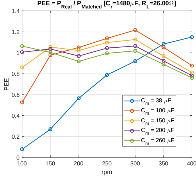
Figure 4.23: Power extraction efficiency (PEE) of the three NVC bridges combined, across the target speed range, for five fixed values of the compensation capacitor C_m ( C_r = 1480 \mu F , R_L = 26.00 \Omega ).
