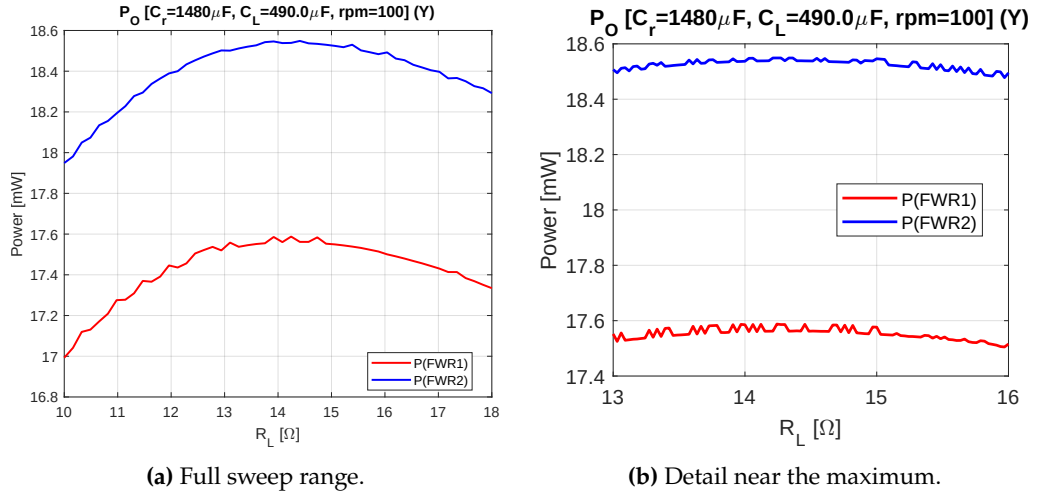
Figure 4.7: Output power of the star-connected first and second bridges as a function of the load resistance R_L at 100 rpm ( C_r = 1480 \mu F , C_m = 490 \mu F ).
