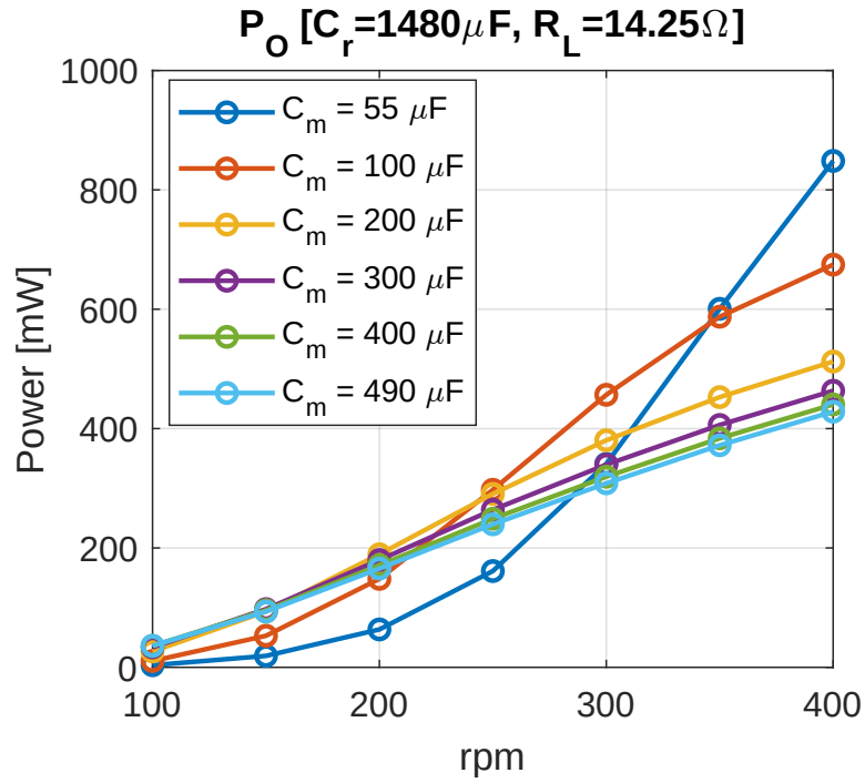
Figure 4.8: Combined output power of the first and second bridges across the target speed range, for six fixed values of the compensation capacitor C_m ( C_r = 1480 \mu F , R_L = 14.25 \Omega ).
