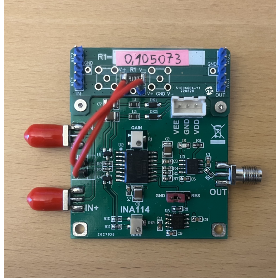
Figure 6.2: One of the six current-sensing boards used in this thesis, built around the INA114AU instrumentation amplifier.
