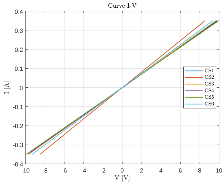
Figure 6.3: Calibration curves of the six current sensors of the MP-VREH, CS1 to CS6.
