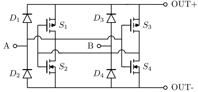
Figure 4.2: Negative voltage converter used for one of the three two-phase groups of pickup units, with input terminals A , B .
