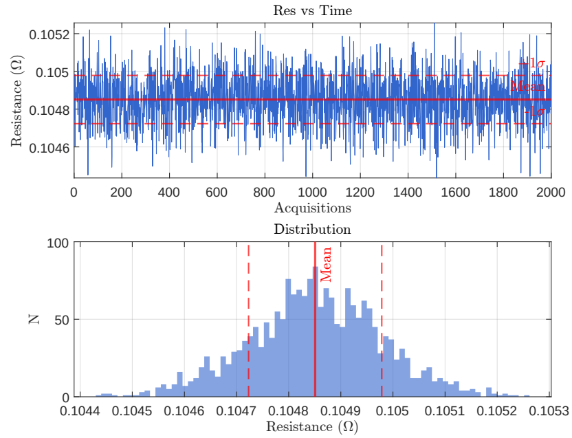
Figure 6.4: 2000 consecutive four-wire measurements of one of the shunt resistors, shown as a representative example of how the repeated measurements are distributed.
