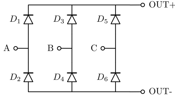
Figure 4.1: Three-phase full-wave bridge rectifier used for one of the two three-phase groups of pickup units, with input terminals A , B , C .
