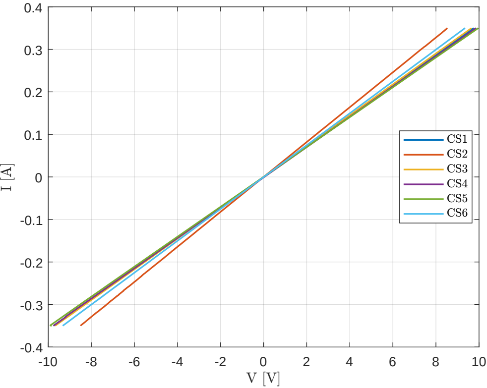
Curve I-V
