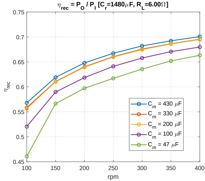
Figure 7.24: Rectifier efficiency \eta_{\text{Rec}} of the three NVC bridges combined, already connected in parallel, across the target speed range, for five fixed values of the compensation capacitor C_m ( C_r = 1480 \mu F , R_L = 6 \Omega ).
