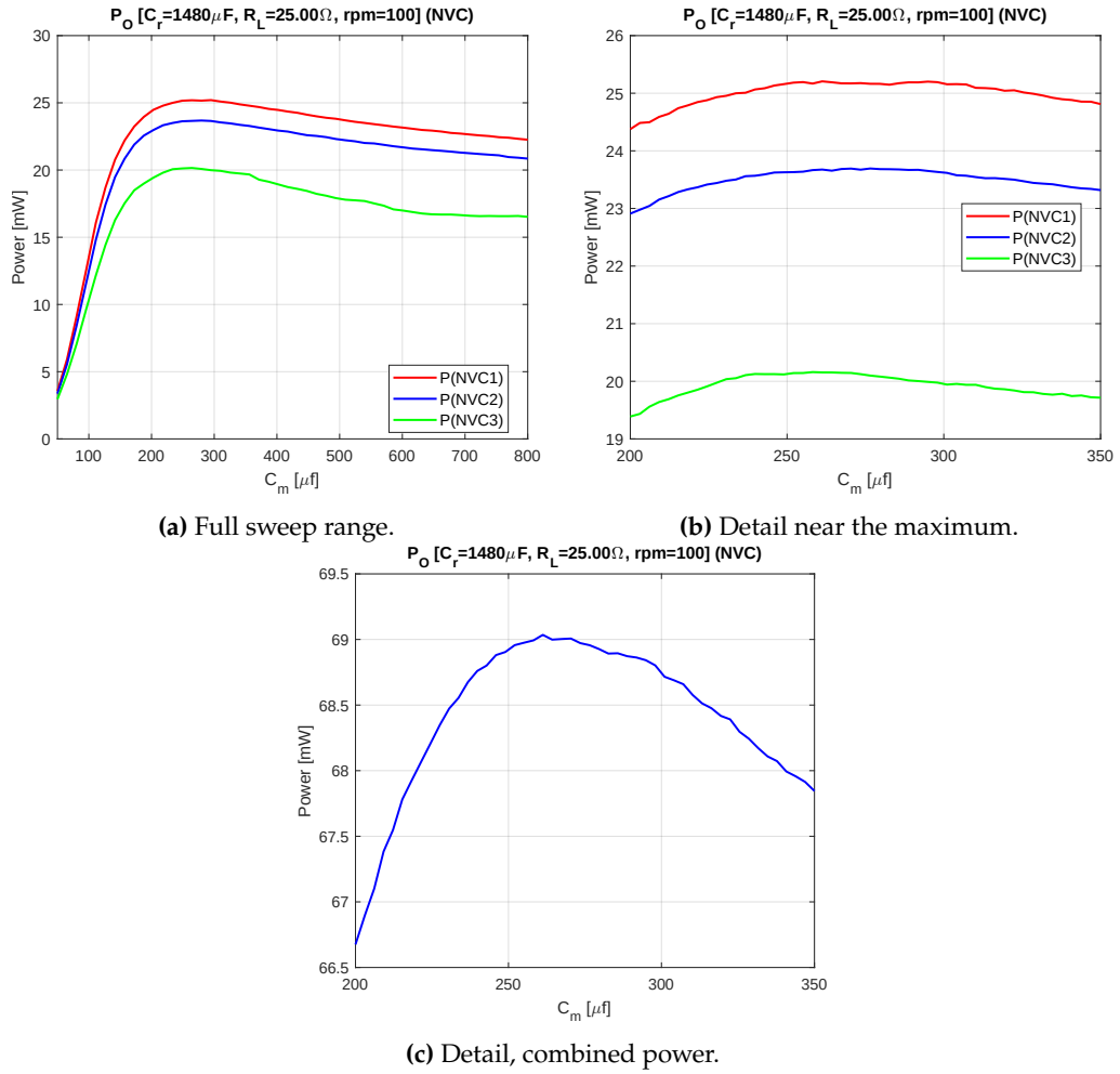
Figure 4.18: Output power of the three NVC bridges as a function of the compensation capacitor C_m at 100 rpm ( C_r = 1480 \mu F, R_L = 25.00 \Omega ), shown individually (a, b) and combined (c).
