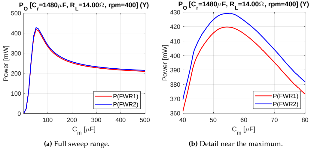
Figure 4.6: Output power of the star-connected first and second bridges as a function of the compensation capacitor C_m at 400 rpm ( C_r = 1480 \mu\text{F} , R_L = 14.00 \Omega ).
