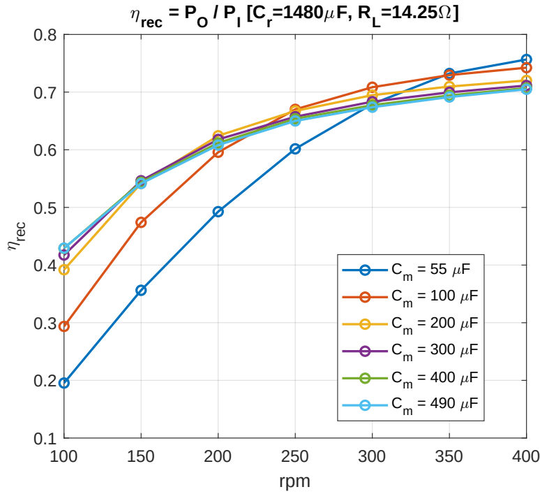
Figure 4.9: Rectifier efficiency \eta_{\text{Rec}} of the first and second bridges combined, across the target speed range, for six fixed values of the compensation capacitor C_m ( C_r = 1480 \mu F , R_L = 14.25 \Omega ).
