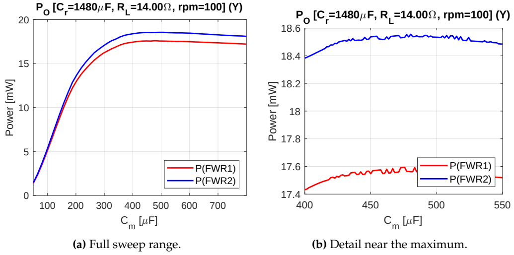
Figure 4.5: Output power of the star-connected first and second bridges as a function of the compensation capacitor C_m at 100 rpm ( C_r = 1480 \mu\text{F} , R_L = 14.00 \Omega ).
