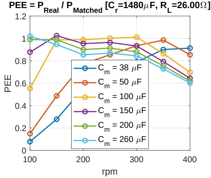
Figure 4.23: Power extraction efficiency (PEE) of the three NVC bridges combined, across the target speed range, for six fixed values of the compensation capacitor C_m ( C_r = 1480 \mu\text{F} , R_L = 26.00 \Omega ).
