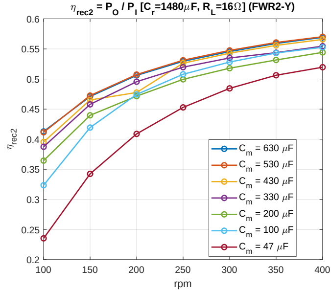
Figure 7.8: Rectifier efficiency \eta_{\text{Rec}} of the second bridge (FWR2) of the star connection across the target speed range, for seven fixed values of the compensation capacitor C_m ( C_r = 1480 \mu\text{F} , R_L = 16 \Omega ).
