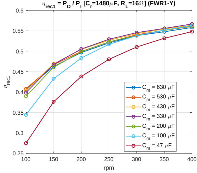
Figure 7.7: Rectifier efficiency \eta_{\text{Rec}} of the first bridge (FWR1) of the star connection across the target speed range, for seven fixed values of the compensation capacitor C_m ( C_r = 1480 \mu\text{F} , R_L = 16 \Omega ).
