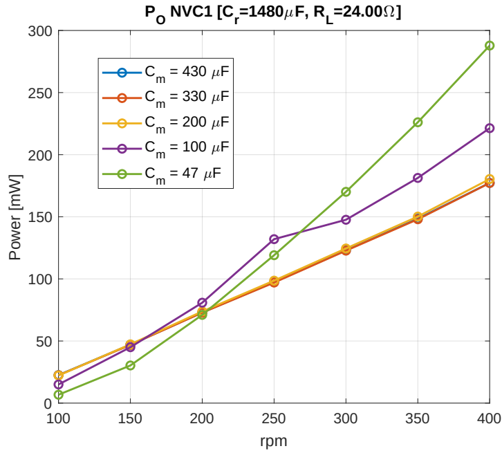
Figure 7.20: Output power of NVC1 across the target speed range, for five fixed values of the compensation capacitor C_m ( C_r = 1480\mu\text{F} , R_L = 24\Omega ).
