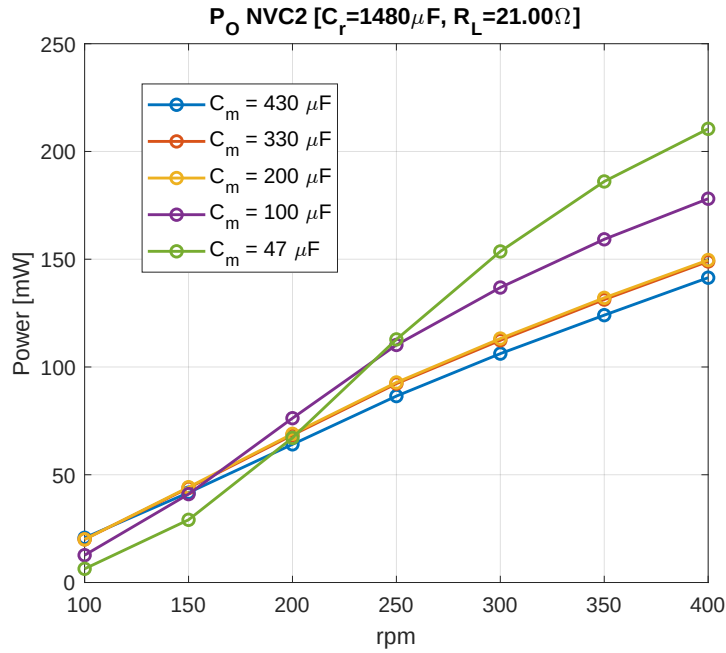
Figure 7.21: Output power of NVC2 across the target speed range, for five fixed values of the compensation capacitor C_m ( C_r = 1480\mu\text{F} , R_L = 21\Omega ).
