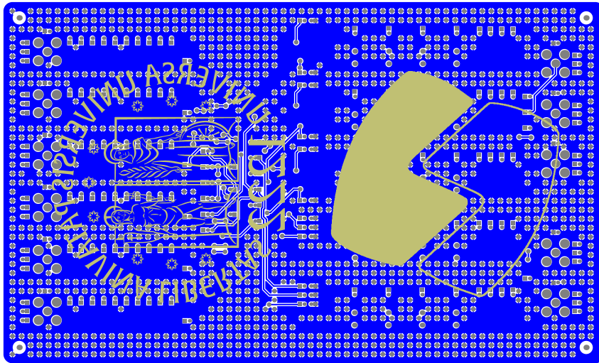
(a) Bottom copper layer.
