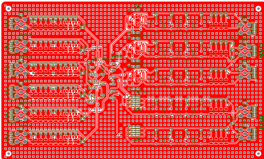
(b) Top copper layer.
