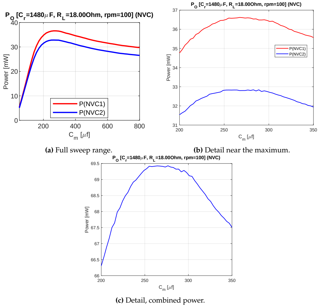
Figure 4.18: Output power of the two NVC bridges as a function of the compensation capacitor C_m at 100 rpm ( C_r = 1480 \mu F, R_L = 18.00 \Omega ), shown individually (a, b) and combined (c).
