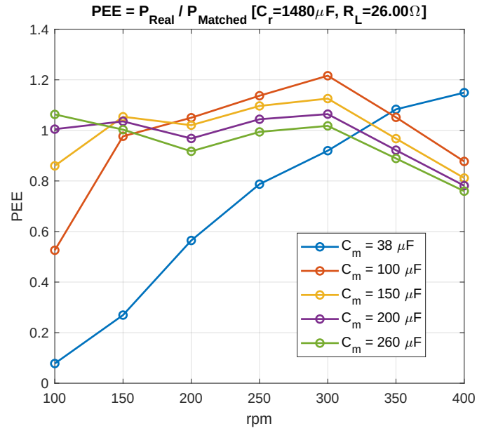
Figure 4.23: Power extraction efficiency (PEE) of the three NVC bridges combined, across the target speed range, for five fixed values of the compensation capacitor C_m ( C_r = 1480 \mu\text{F} , R_L = 26.00 \Omega ).
