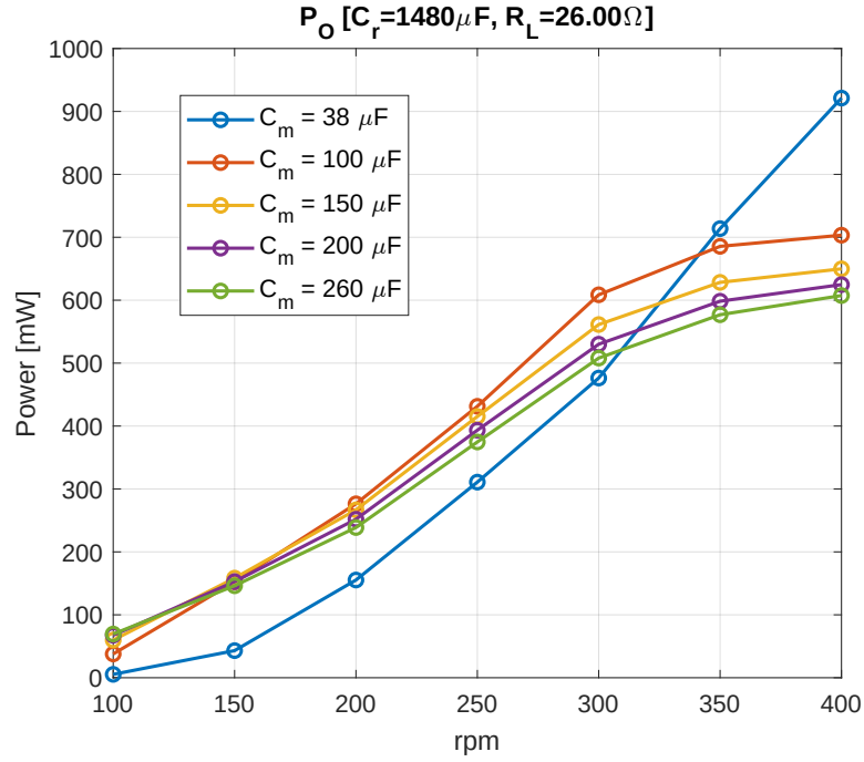
Figure 4.21: Combined output power of the three NVC bridges across the target speed range, for five fixed values of the compensation capacitor C_m ( C_r = 1480 \mu F , R_L = 26.00 \Omega ).
