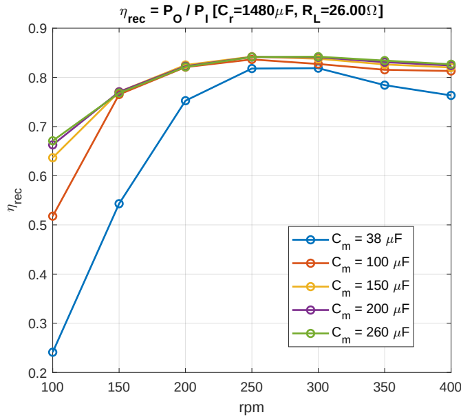
Figure 4.22: Rectifier efficiency \eta_{\text{Rec}} of the three NVC bridges combined, across the target speed range, for five fixed values of the compensation capacitor C_m ( C_r = 1480 \mu\text{F} , R_L = 26.00 \Omega ).
