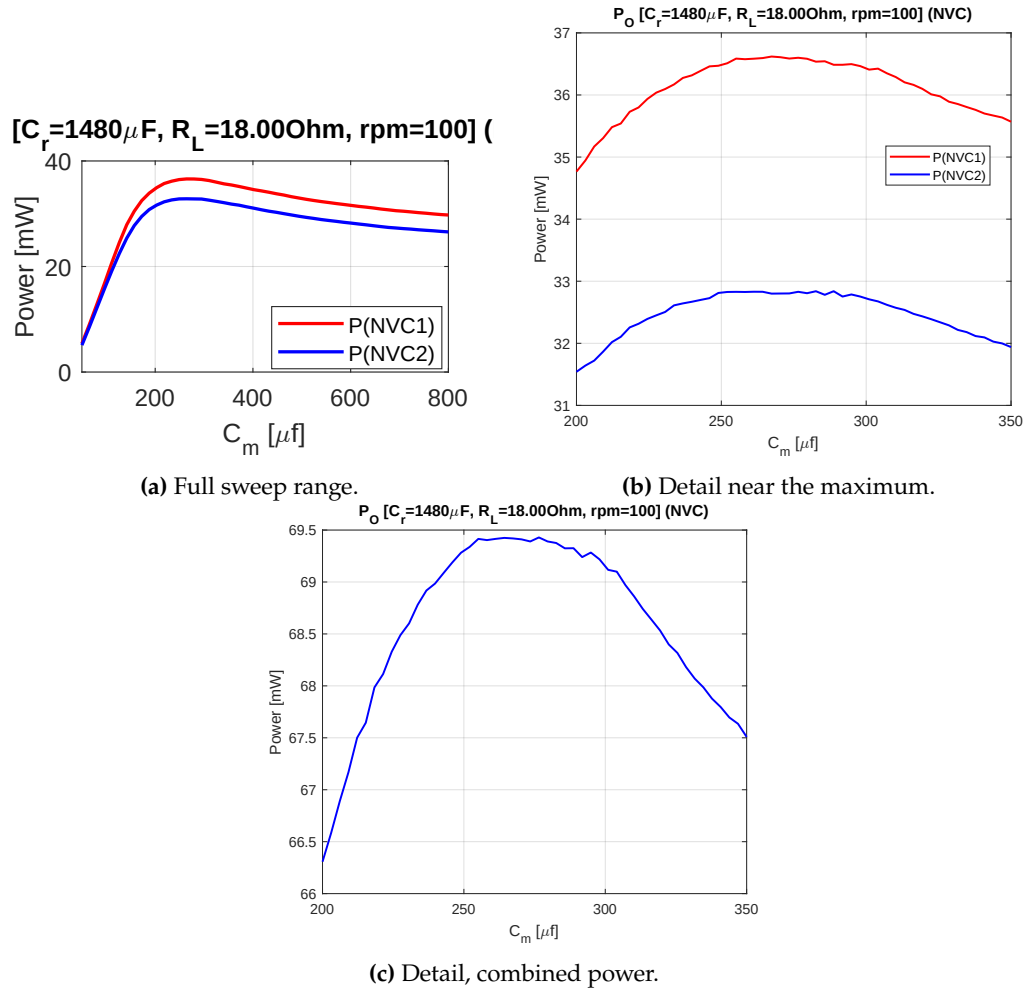
Figure 4.18: Output power of the two NVC bridges as a function of the compensation capacitor C_m at 100 rpm ( C_r = 1480 \mu\text{F} , R_L = 18.00 \Omega ), shown individually (a, b) and combined (c).
