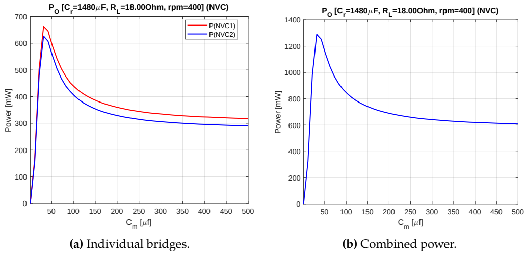
Figure 4.19: Output power of the two NVC bridges as a function of the compensation capacitor C_m at 400 rpm ( C_r = 1480 \mu\text{F} , R_L = 18.00 \Omega ), shown individually (a) and combined (b).
