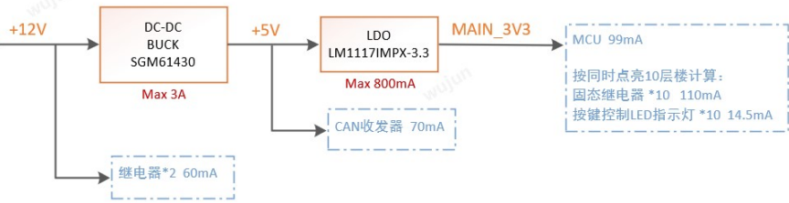
Power tree
