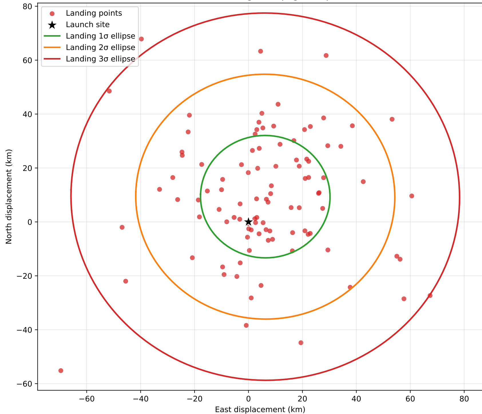
Monte Carlo landing and apogee dispersion
