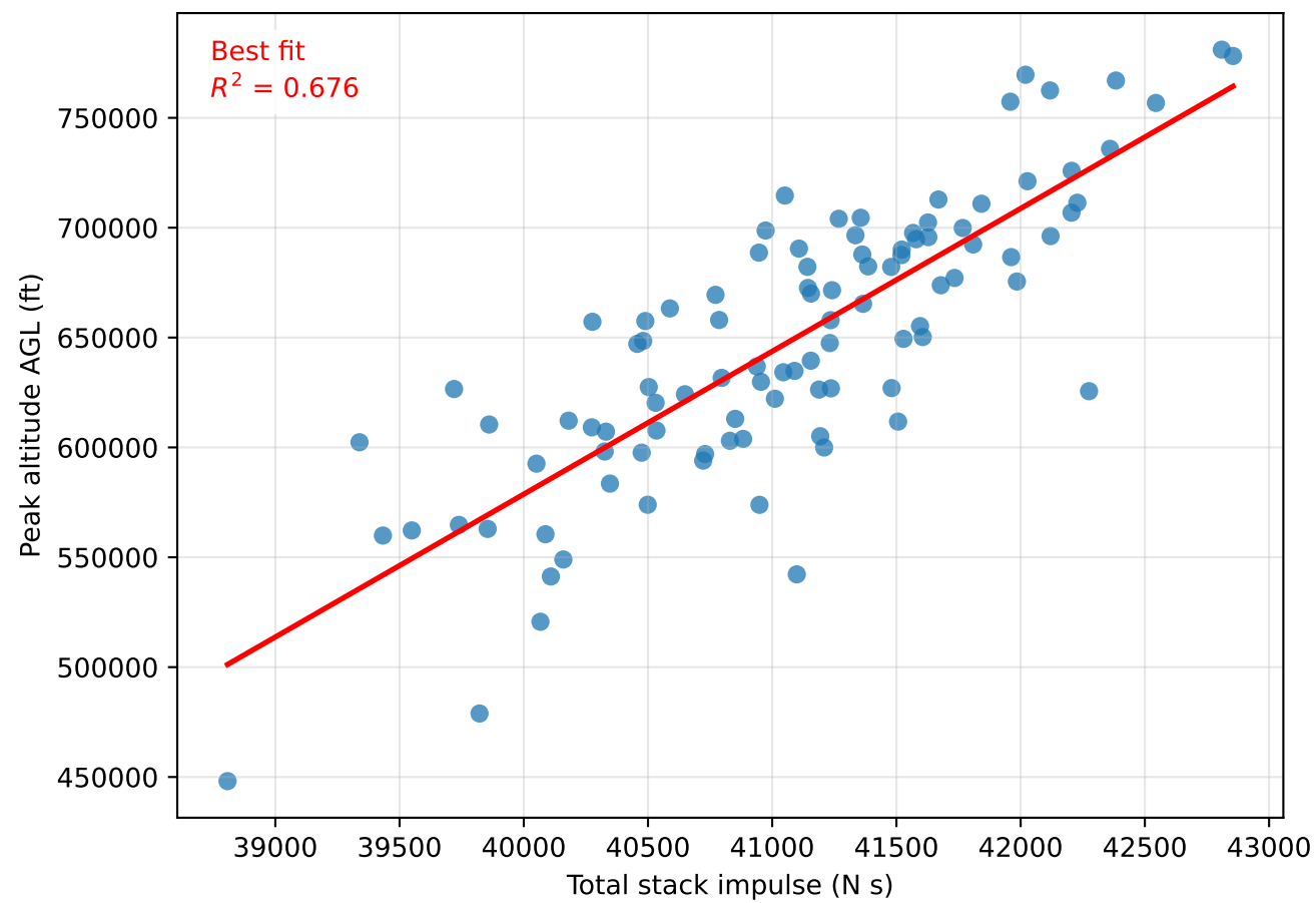
Stage impulse and mass sensitivity of apogee
