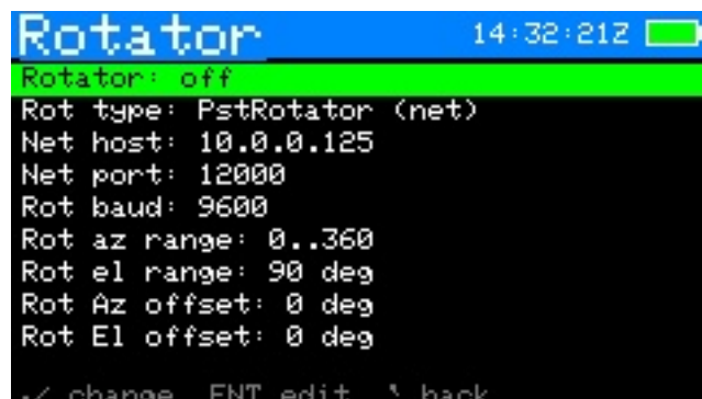
Figure 35: Settings — Rotator
