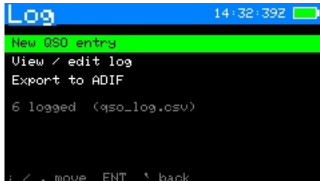
Figure 38: Log menu
