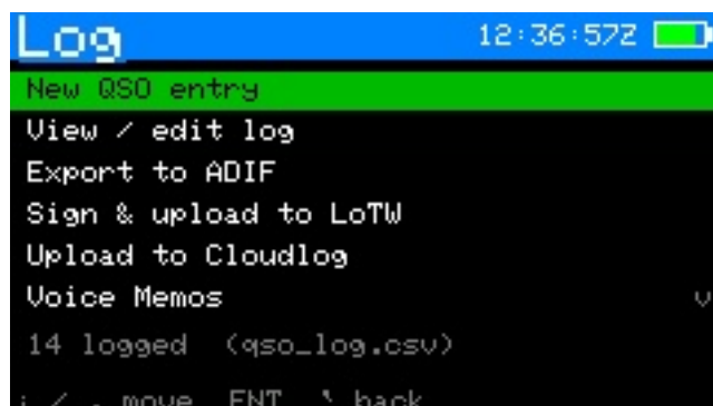
Figure 54: Log menu
