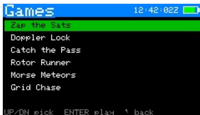
Figure 74: Games menu
