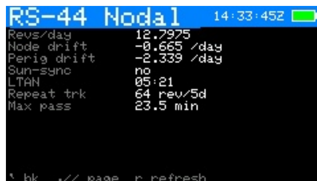
Figure 8: Orbital analysis — Nodal
