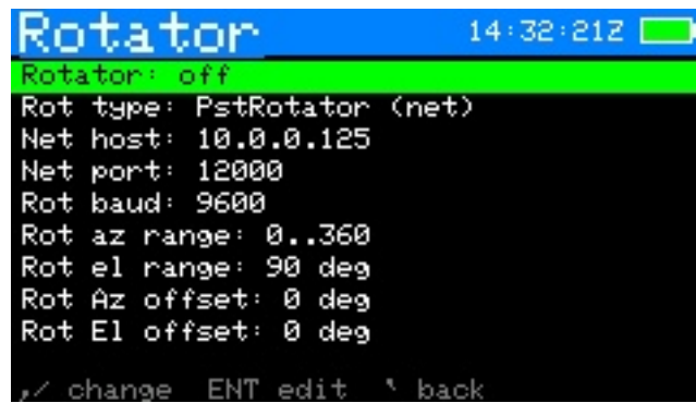
Figure 35: Settings — Rotator
