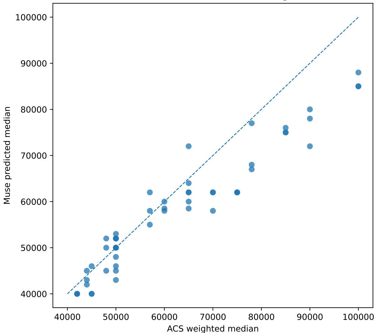
Predicted vs ACS median — wages
