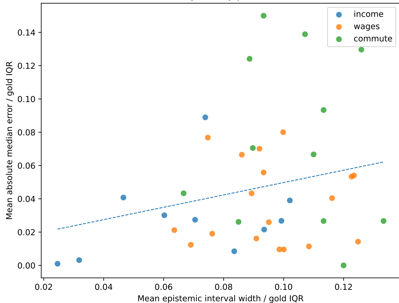
Stated uncertainty weakly predicts actual error
