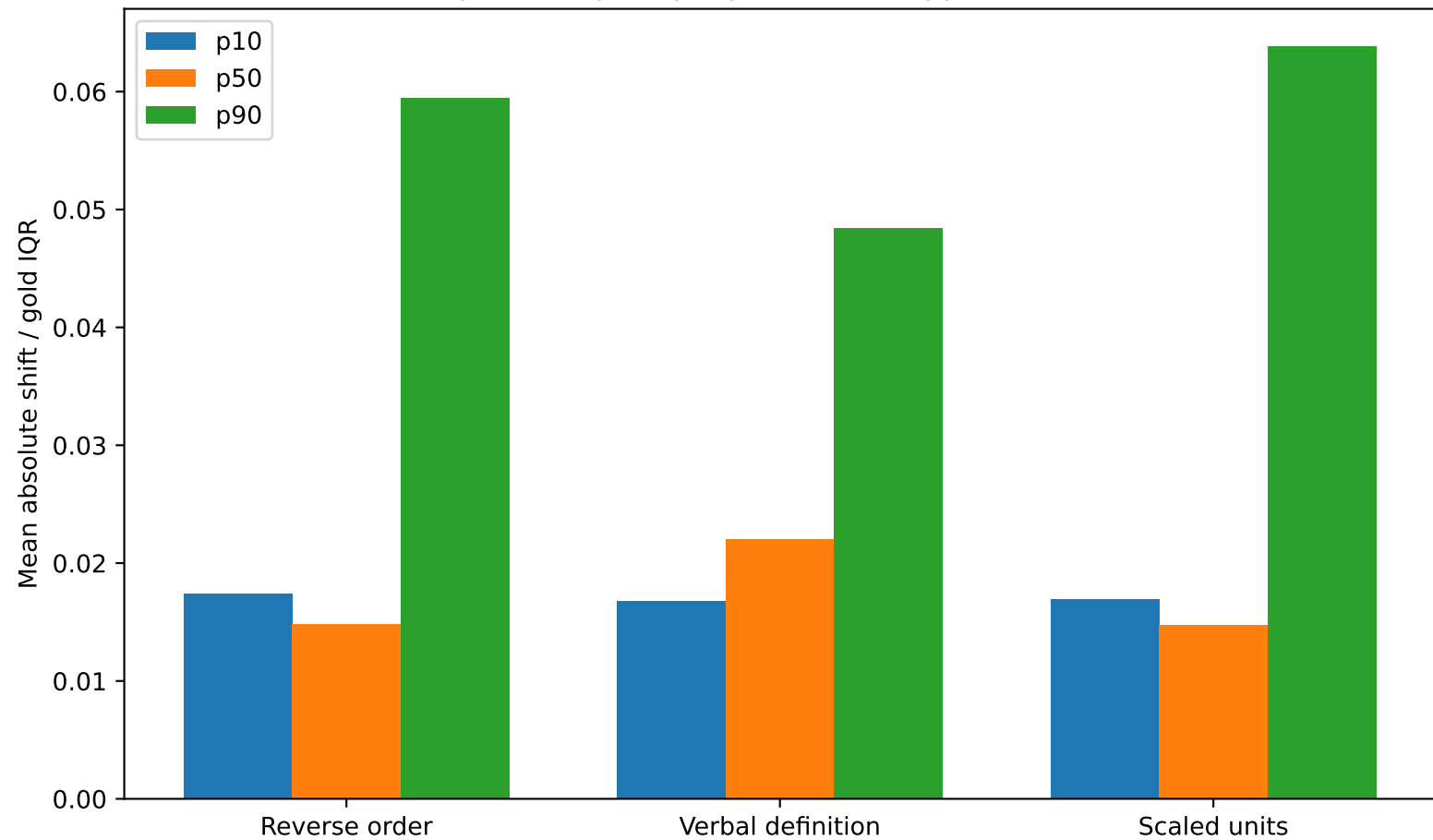
Equivalent prompts perturb the upper tail most
