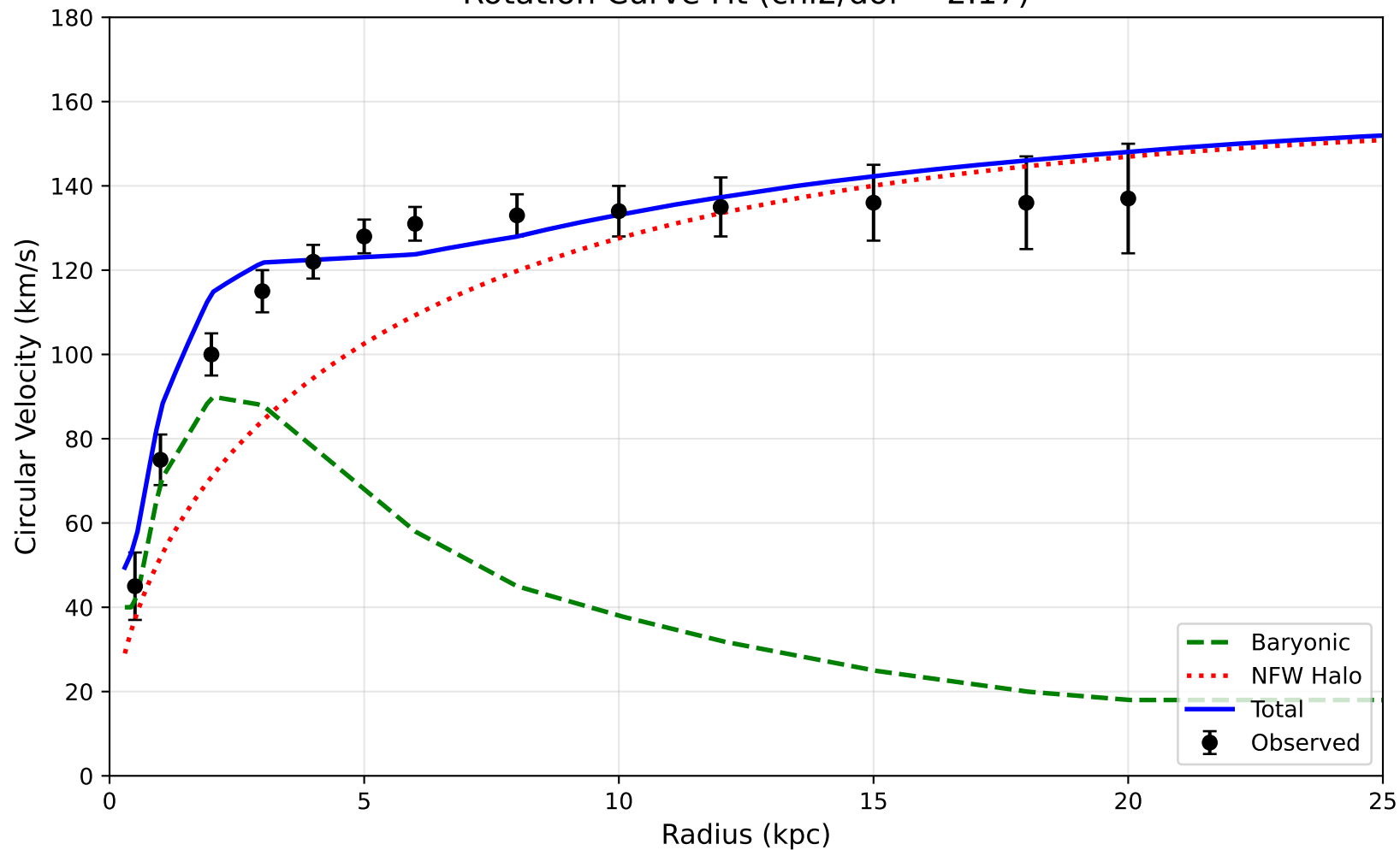
Rotation Curve Fit ( \chi^2/\text{dof} = 2.17 )
