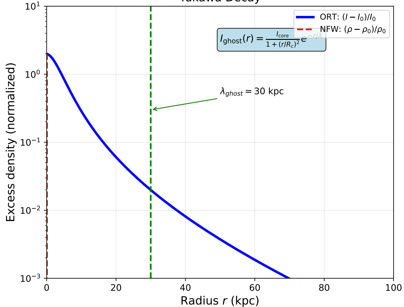
Full Range (Log Scale) Yukawa Decay
