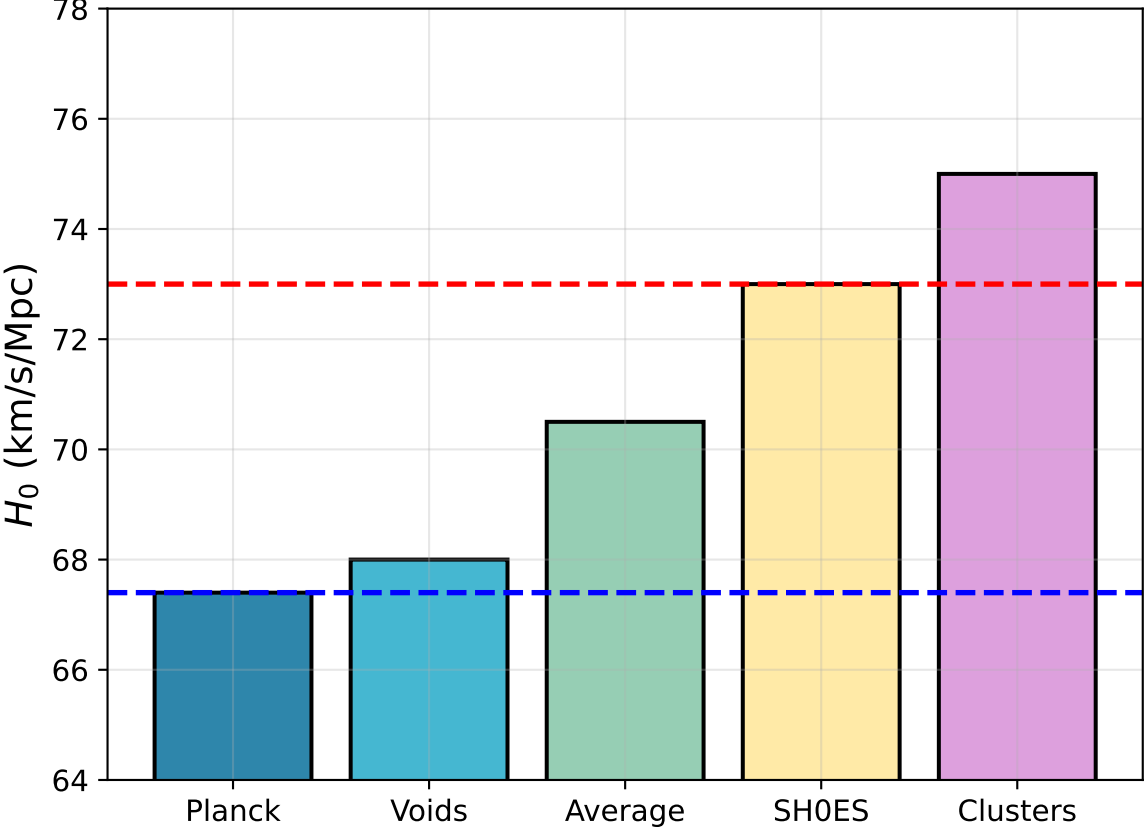
(A) Hubble Tension Resolution
