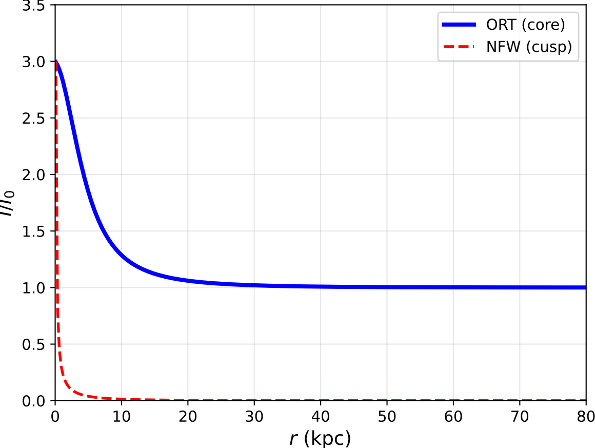
(C) Ghost Halo Profile
