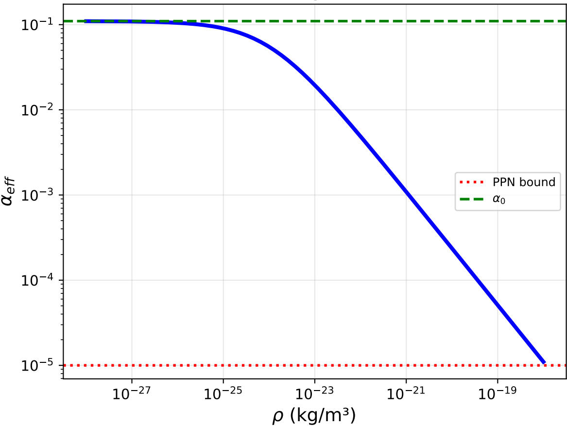
(B) Screening Mechanism
