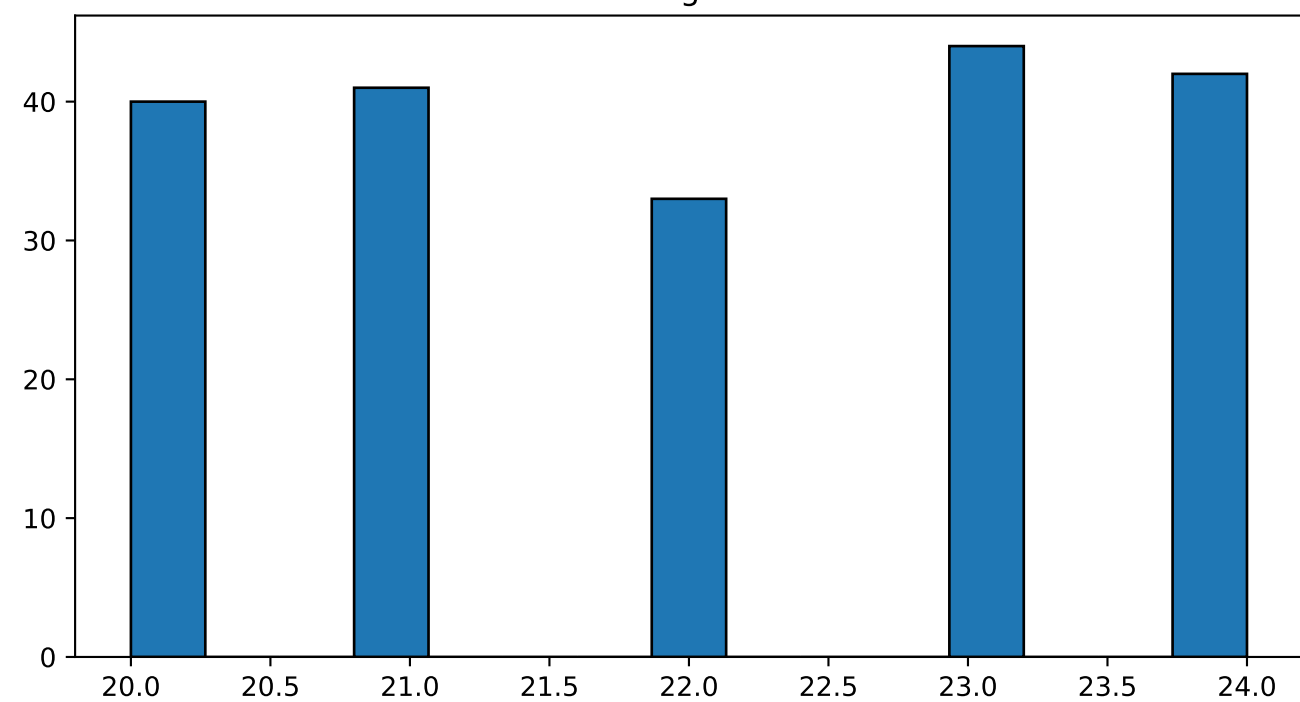
Communication_Skills
