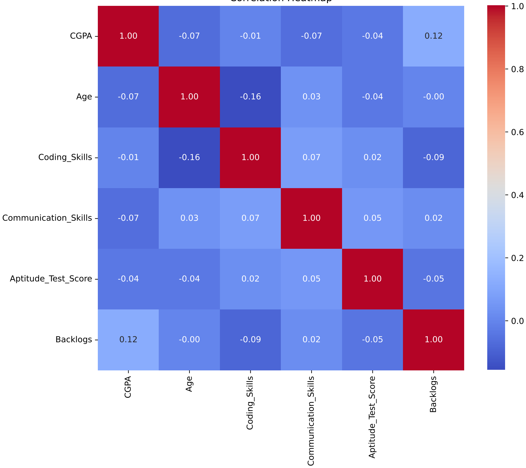
Correlation Heatmap
