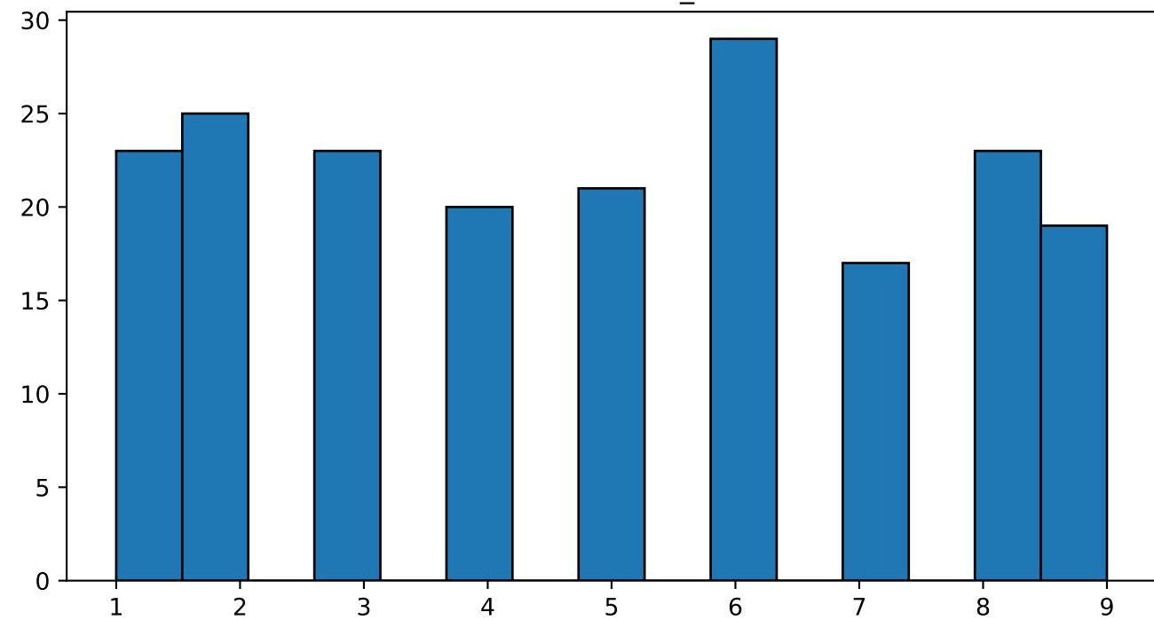
Backlogs
