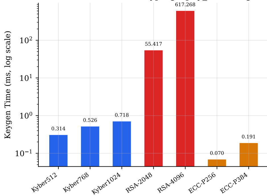
(b) Raspberry Pi 4B — Cortex-A72 @ 1.8 GHz (OQS benchmark + cryptography_lib timings)
