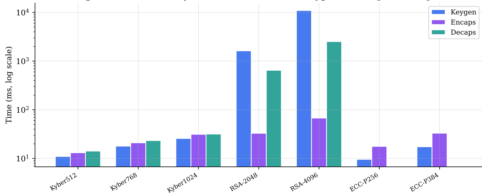
Figure 2: Full KEM Cycle — STM32F446RE (keygen + encaps + decaps)
